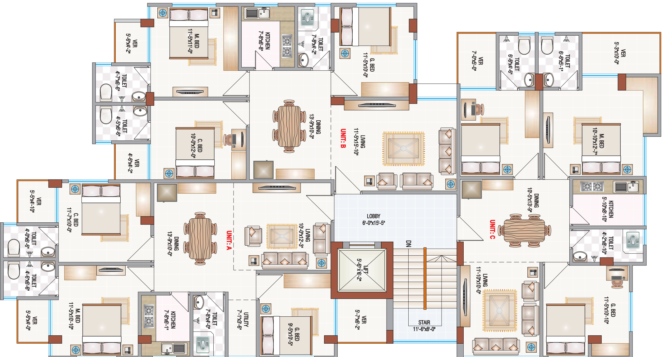
1ST TO 7TH FLOOR PLAN (APARTMENT)
